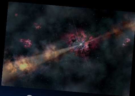
Space Plasma
