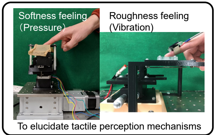
Tactile display device
