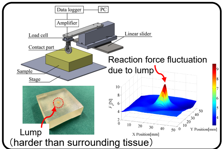
Medical tactile sensor system
