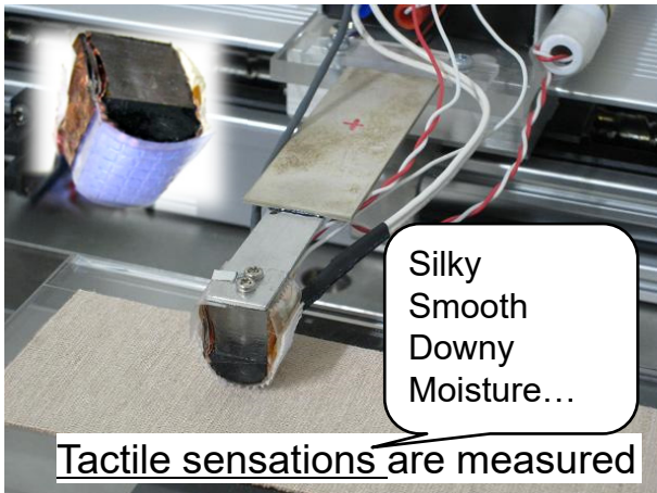
Intelligent finger system
