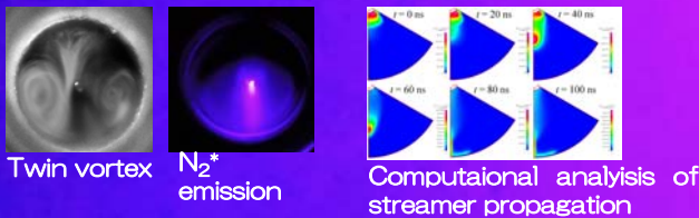
Twin vortex N 2 * emission Computational analysis of streamer propagation
